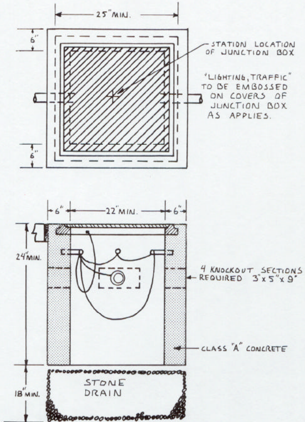
SECTION A-A - TYPE II
